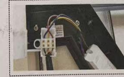
11、Wiring for driving input line and ground line. Lock nut corresponding to box
